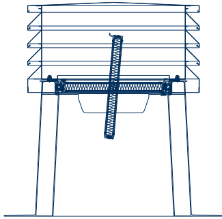
BK-TF 450 - 1 Lamelle
