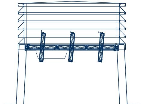
BK-TF 800 - 3 Lamellen
