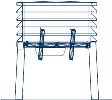
BK-TF 600 - 2 Lamellen
